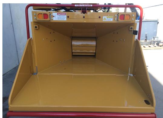
The RC1220 boasts an impressive 30.5 x 50.8cm in-feed opening.
