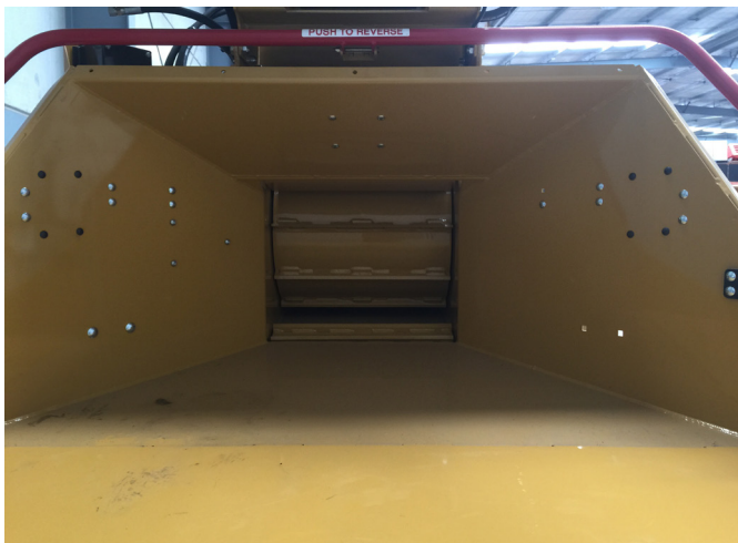
Large Feed Table with 18-inch (45.7cm) x 24-inch (61cm) Infeed Opening
